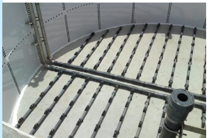
Aeration system
